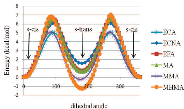
Figure 2. Rotational potential (kcal/mol) as a function of the dihedral angle ( C_1C_2C_3C_4O_7 ) for monomers M1–M6.
