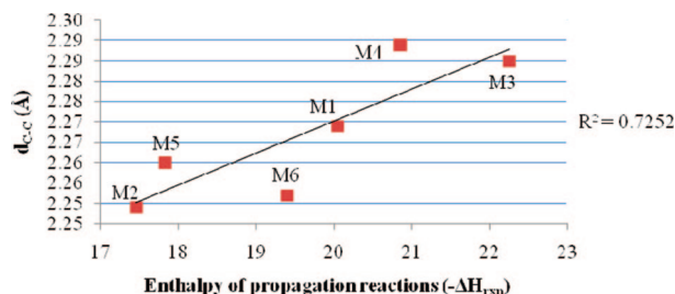
Figure 9. Dependence of the C...C bond distance on the heat of reaction ( -\Delta H_{\text{rxn}} ) in the transition states of the dimeric radicals (MPWB1K/6-311+G(3df,2p)//B3LYP/6-31+G(d)).
